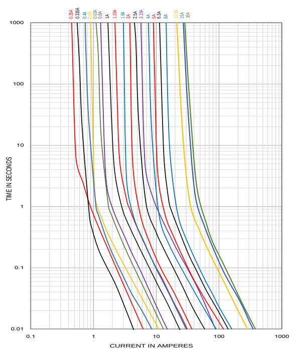
Average Current Curve (I-T Curve)
