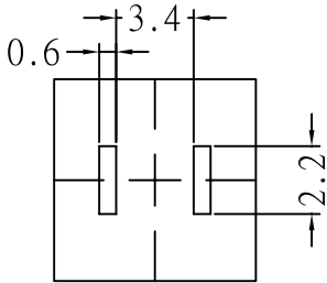
PCB MOUNTING
