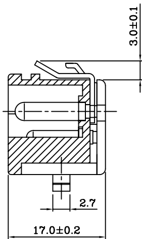
B-B SECTION
