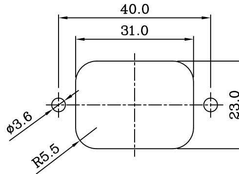
REAR MOUNTING
